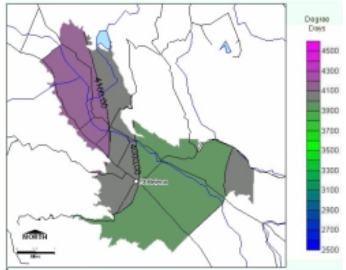
St. Helena AVA 1997 Growing Degree Day Map
